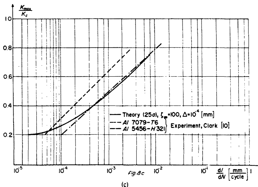
Fig. 8. Comparison of the experimental data on fatigue collected by Cherepanov[7], Clark[10], Forman[11] and the theoretical data derived from the present investigation.
